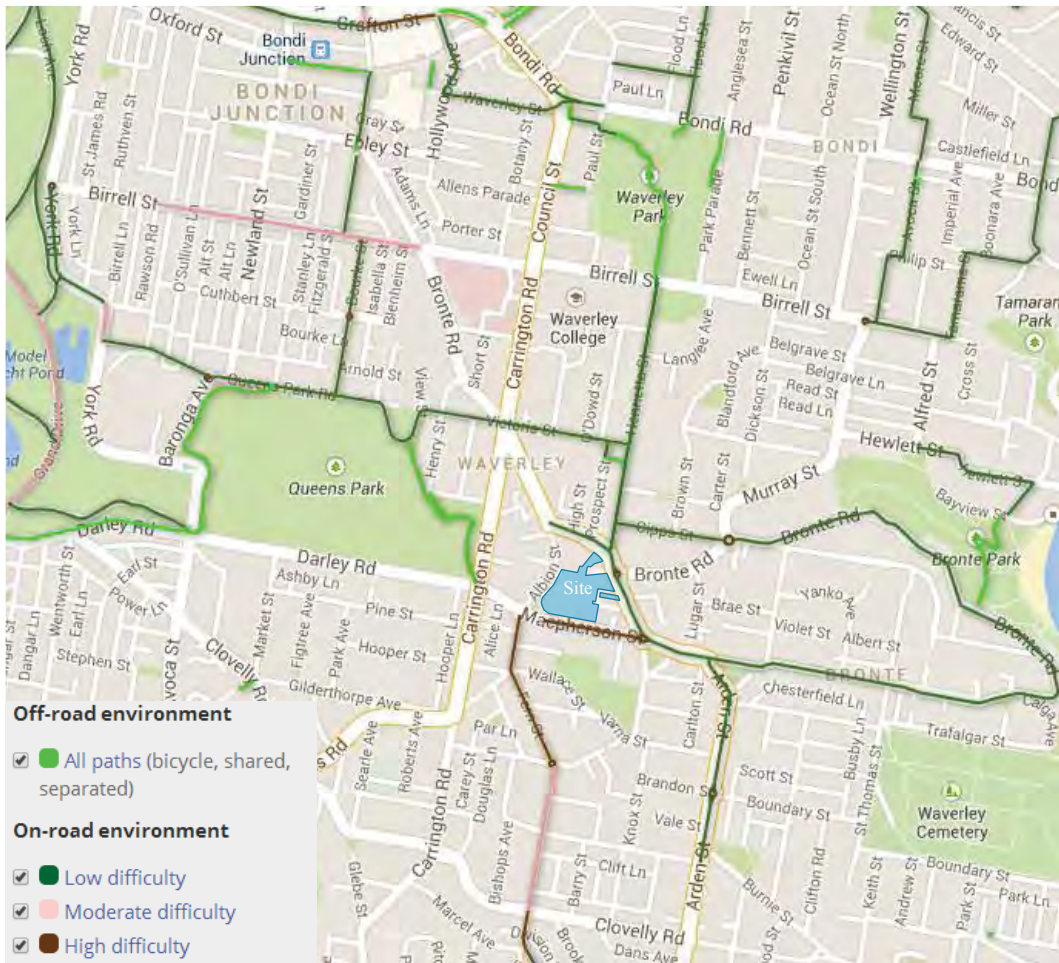
Figure 23: Bicycle network
